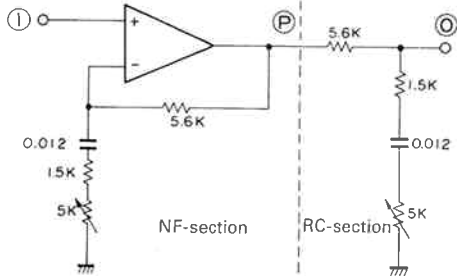
Fig. 4-1 Equivalent circuit for flat TREBLE
