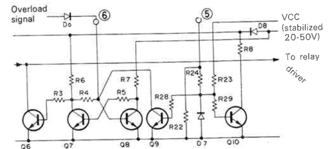
Fig. 12 Overload detector/Line voltage detector
