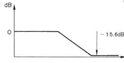
Fig. 5-2 Frequency responses of NF-section (above) and RC-section (below)
